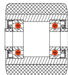
Labyrinth sealing
