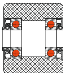
Labyrinth sealing
