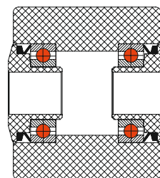
V-ring sealing gasket
