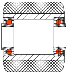
ZZV-ball bearing
