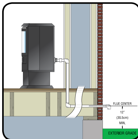
Single Vent Downward and Out
