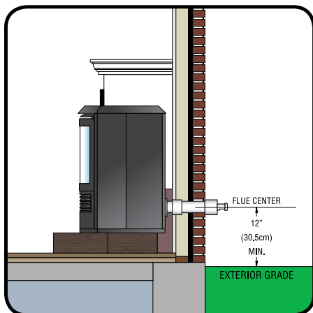
Co-axial Straight Out Venting
