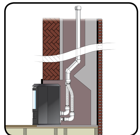
Co-linear Vertical Termination
